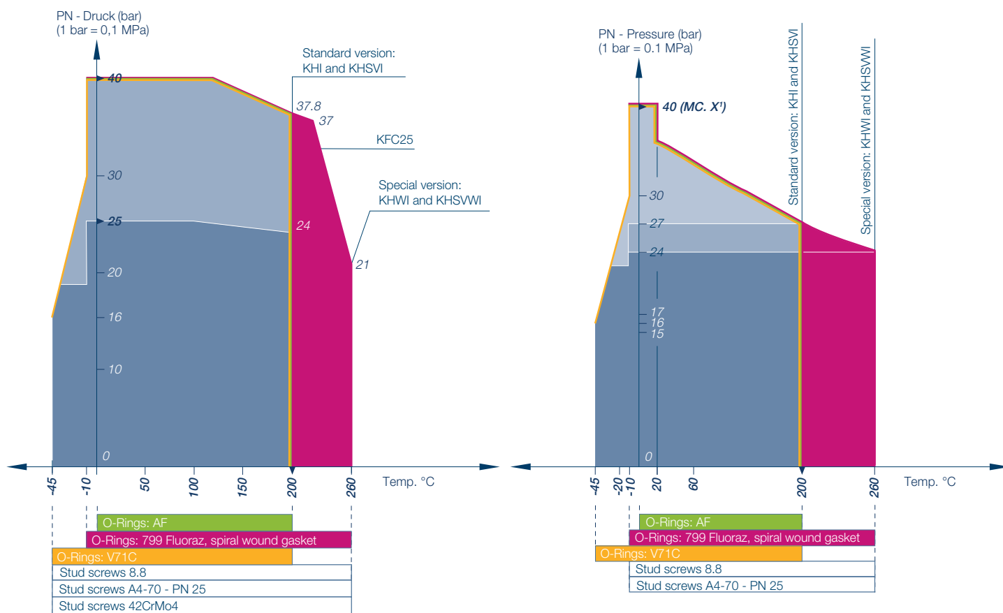
Steel casting Material code VII
